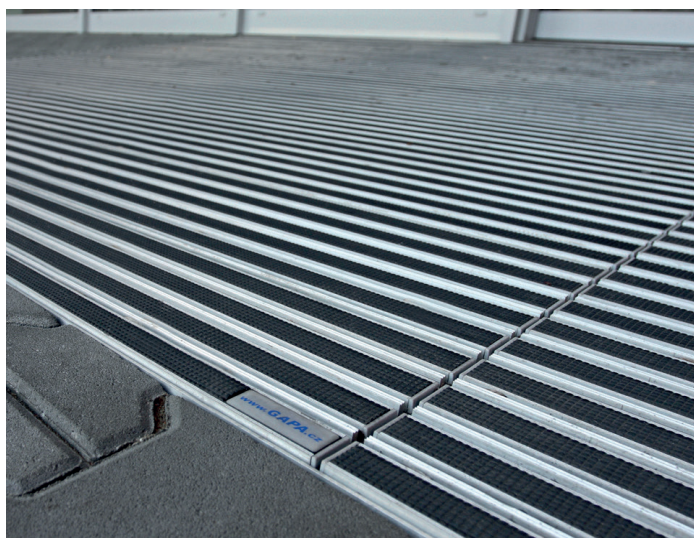
grooved PVC / aluminium scraper / textile
